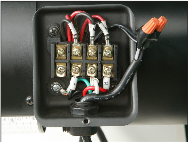
Figure 69. Motor wiring.
